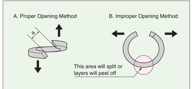
Fig. 5 Proper Installation
